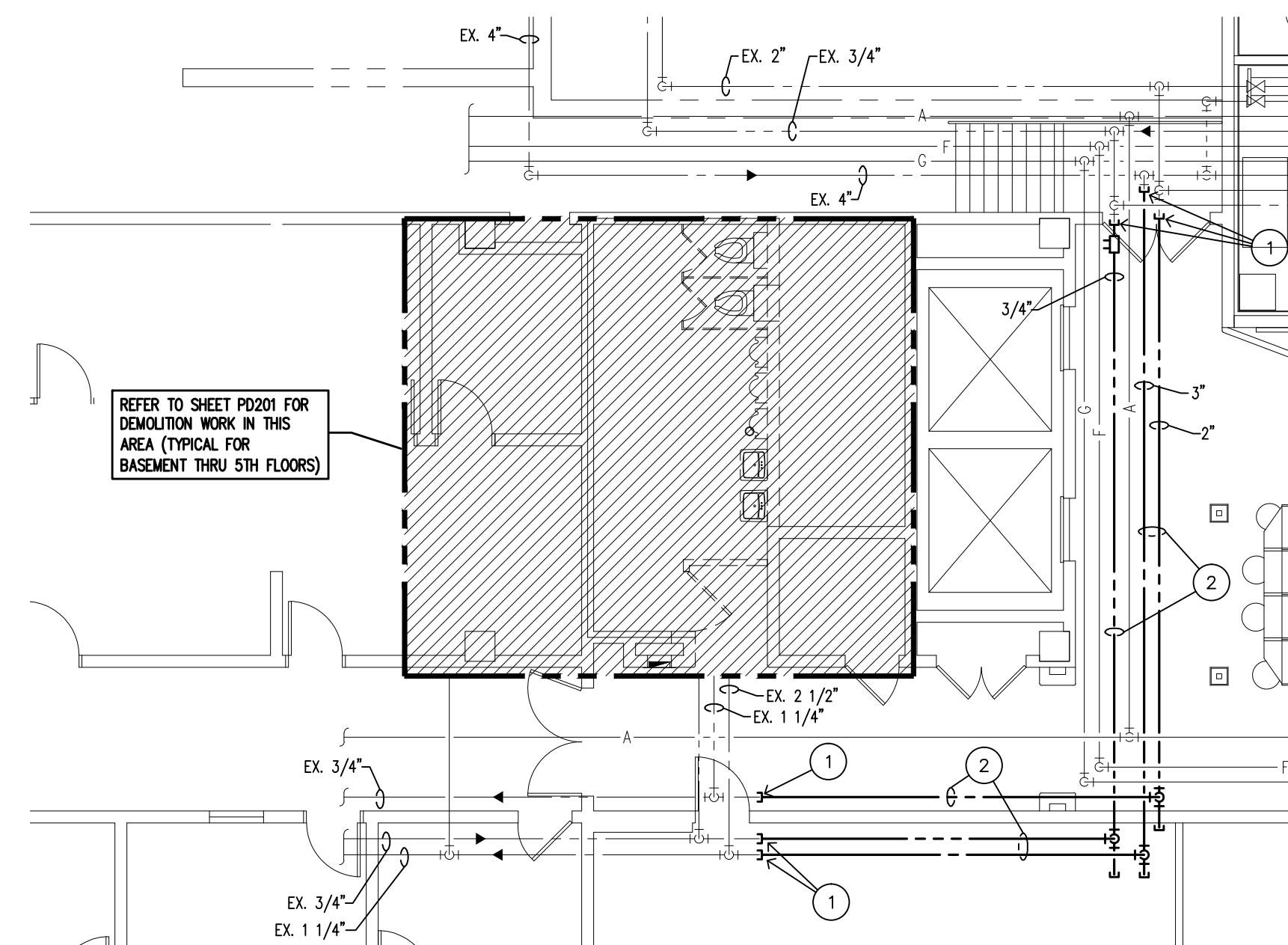
PARTIAL BASEMENT FLOOR PLAN (BASE BID) - PLUMBING DEMOLITION
